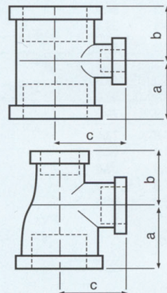
FIG. 130R RED. TEES (RT)
