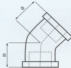
FIG. 121 STREET ELBOWS 45° (SL 45)
